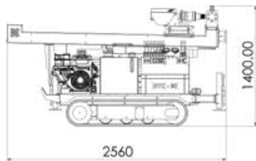
SIDE VIEW - MAX HEIGHT
